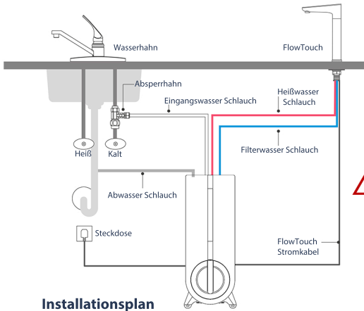
Installationsplan
